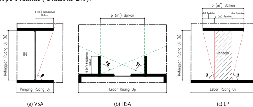
Gambar 3 (a) Vertical Shading Angel (VSA) , (b) Horizontal Shading Angle , (c) End Profile (EP)
