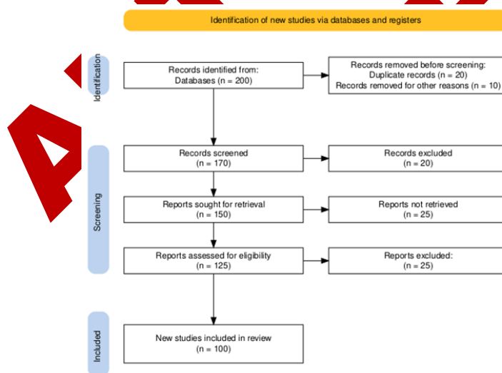
Gambar 1. Flowchart PRISMA
