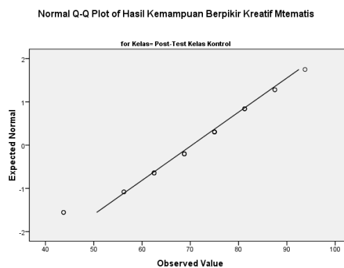
Gambar 3. Grafik normal q-q plot post-test
