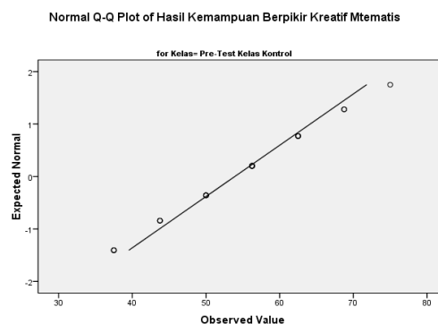
Gambar 2. Grafik normal q-q plot pre-test
