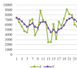
Gambar 3. Grafik Peramalan Single Exponential Smoothing
