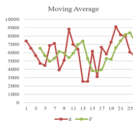
Gambar 3. Grafik Peramalan Moving Average
