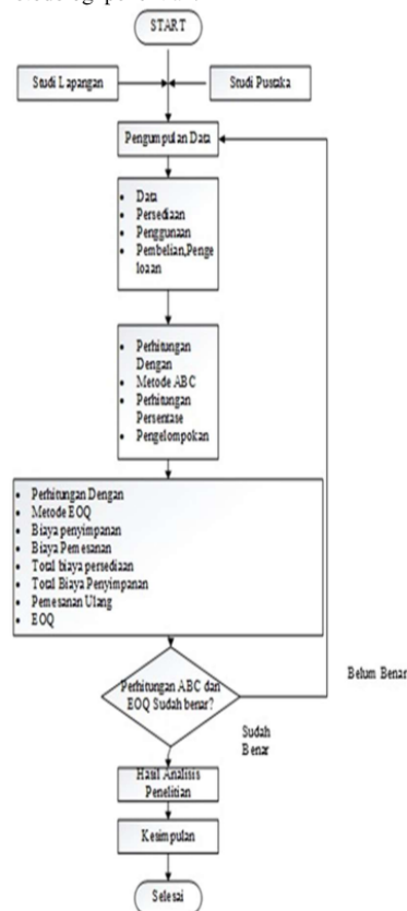
Gambar 4 Flowchart
