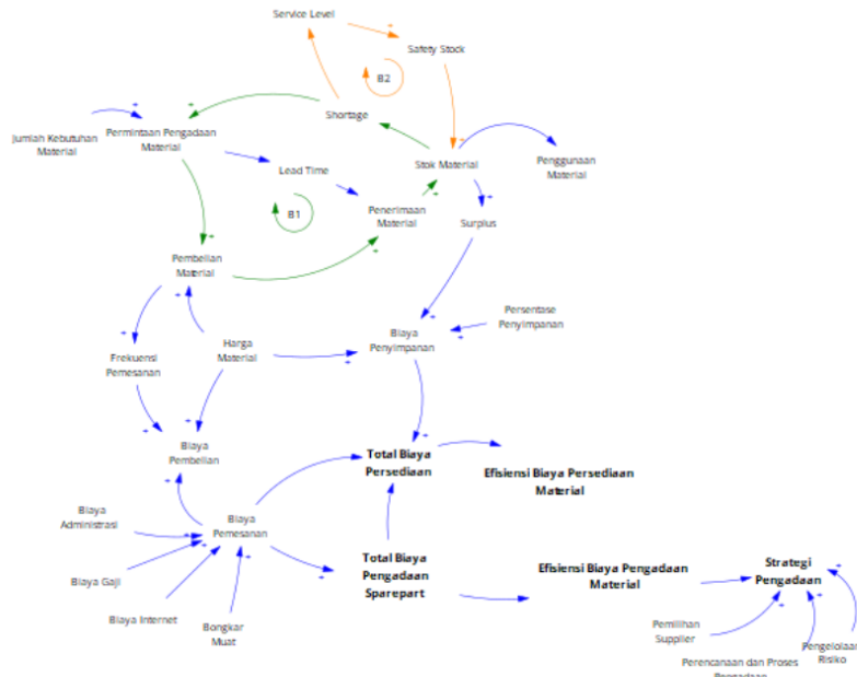
Gambar 2. Causal Loop Diagram Sistem Pengadaan Material
